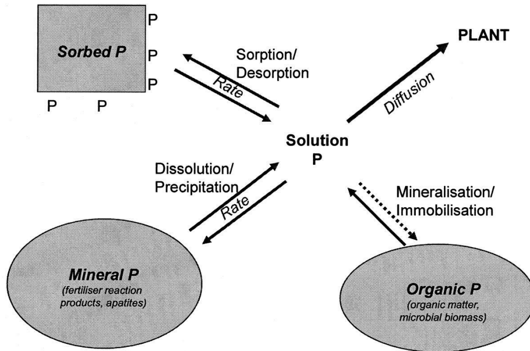
Fig. 1. Soil phosphorus pools and processes.
